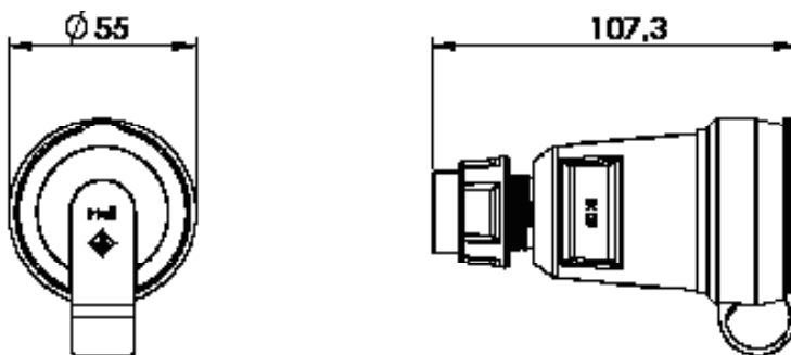
Dimensional drawing – connector with self-closing hinged lid
