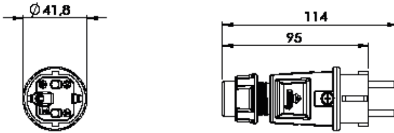
Dimensional drawing – connector
