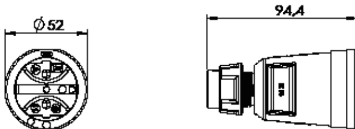
Dimensional drawing – connector with collar
